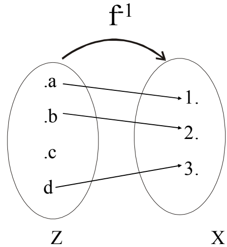
INVERSE
