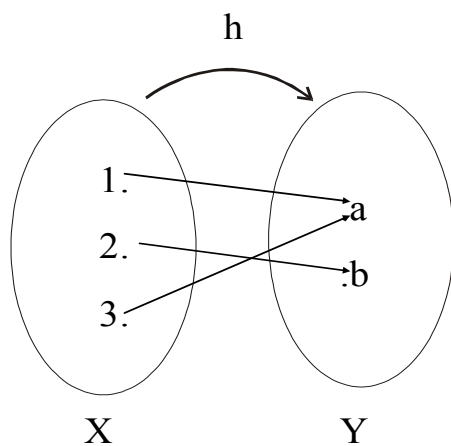
SURJECTIVE FUNCTION
